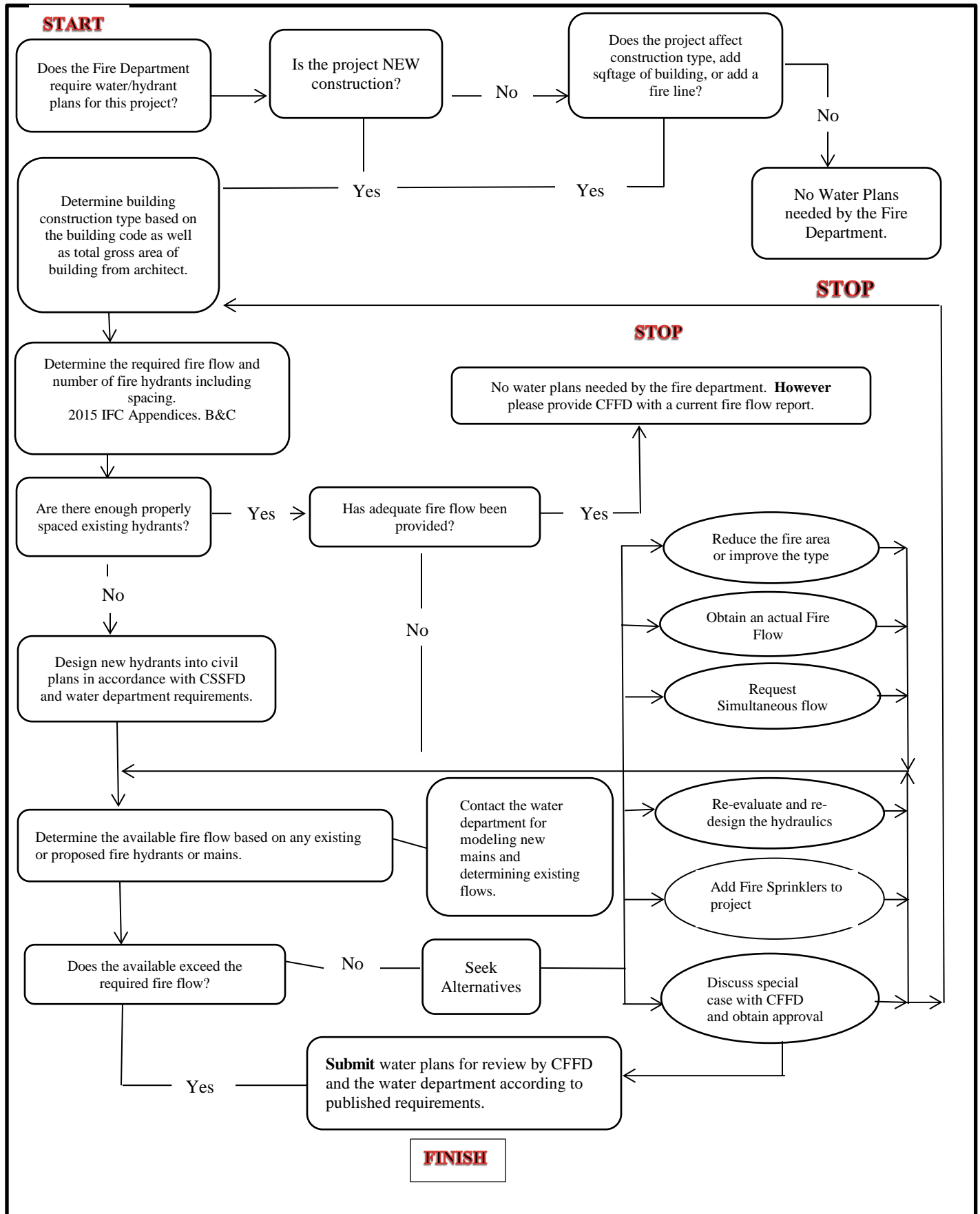
Procedural Flow Chart for Water Plan Submitted to Fire Prevention Division
